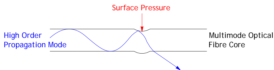
Diagram 1: Microbending
